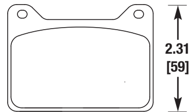
WILWOOD 7912
