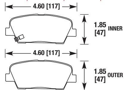
HYUNDAI (REAR)
