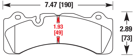
BREMBO SPORT BIG BRAKE KIT SCALLOPED
