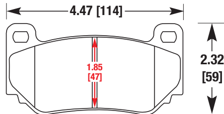
AP RACING CP7600D46
