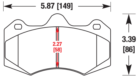
AP RACING CP7040D61
