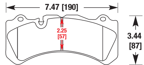
BREMBO SPORT BIG BRAKE KIT
