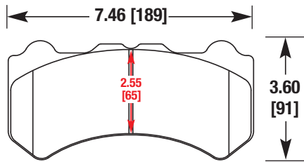
NISSAN
