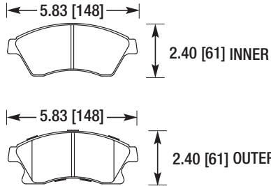
CHEVY CRUZE/SONIC
