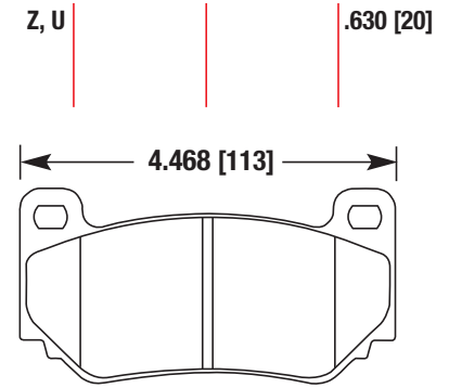
AP RACING CP7600D46
