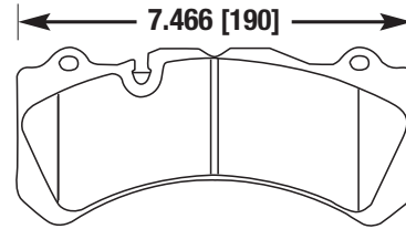
BREMBO SPORT BIG BRAKE KIT
