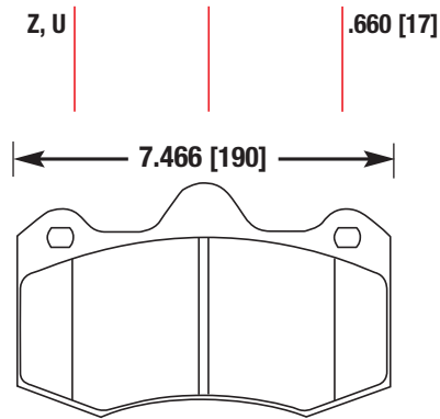
AP RACING CP6600D55
