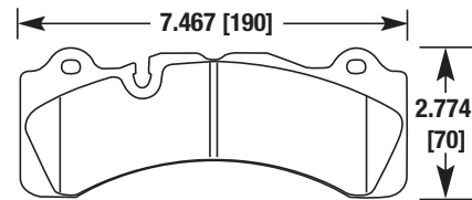
BREMBO SPORT BIG BRAKE KIT SCALLOPED
