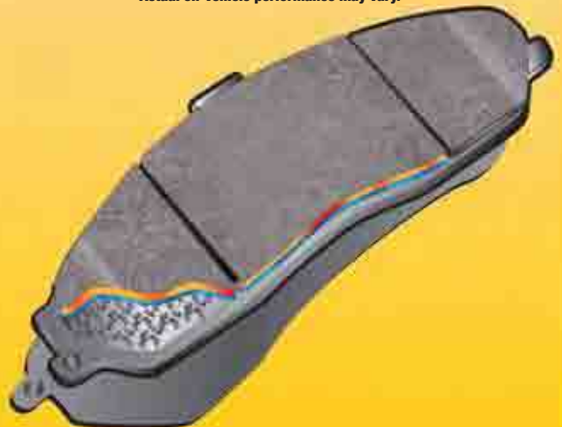
Results based on A04D Dyno tests using D52 automotive platform. Actual on-vehicle performance may vary.
